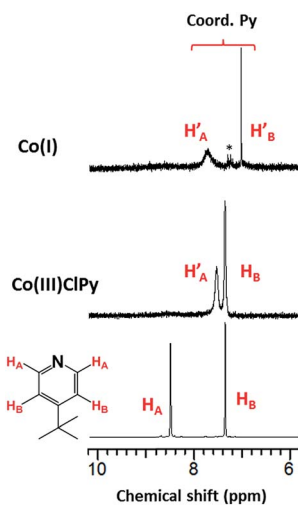
Fig. 11 1 H-NMR spectra of [Co I (prdioH)( 4t Bu 4 py)], in CD 3 CN. The asterisk denotes the presence of adventitious toluene. See ESI† for the complete spectra.
