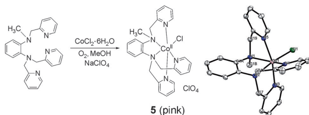
Figure 3. Synthesis of \text{Co}^{\text{II}} complex 5 and its ORTEP representation at 50% ellipsoid probability.
