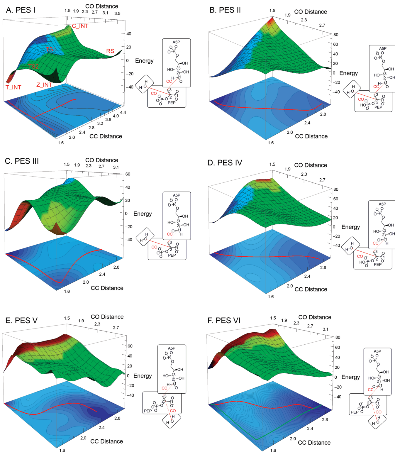
FIGURE 2: (A) PES I, reaction in which \text{O}^{\text{WAT}} attacks the si side of \text{C}2^{\text{PEP}} and \text{C}3^{\text{PEP}} attacks the re side of \text{C}1^{\text{A}5\text{P}} ; PEP phosphate is deprotonated. (B) PES II, same as (A) but with PEP phosphate partially protonated. (C) PES III, reaction in which \text{O}^{\text{WAT}} attacks the si side of \text{C}2^{\text{PEP}} and \text{C}3^{\text{PEP}} attacks the si side of \text{C}1^{\text{A}5\text{P}} ; PEP phosphate is deprotonated. (D) PES IV, same as (C) but with PEP phosphate partially protonated. (E) PES V, reaction in which \text{O}^{\text{WAT}} attacks the re side of \text{C}2^{\text{PEP}} and \text{C}3^{\text{PEP}} attacks the re side of \text{C}1^{\text{A}5\text{P}} ; PEP phosphate is deprotonated. (F) PES VI, reaction in which \text{O}^{\text{WAT}} attacks the re side of \text{C}2^{\text{PEP}} and \text{C}3^{\text{PEP}} attacks the si side of \text{C}1^{\text{A}5\text{P}} ; PEP phosphate is deprotonated. CC and CO distances are in Å; energies are in kcal/mol. Colors on the PESs represent in a qualitative way proton movements along the reaction path: green for proton on \text{O}^{\text{WAT}} , blue for proton nearing \text{O}1^{\text{A}5\text{P}} , and red for proton nearing PEP phosphate oxygen. Colors on the projected contours below the PESs reflect energy levels, with darker shades of blue corresponding to lower energy.
