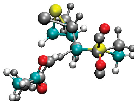
FIGURE 7: Comparison between the TS for syn elimination in solution (structure in gray, dihedral angle -34^\circ ) and TS for syn elimination with the same dihedral angle as in the MMP2 active site (structure in color, dihedral angle as 45^\circ ).
