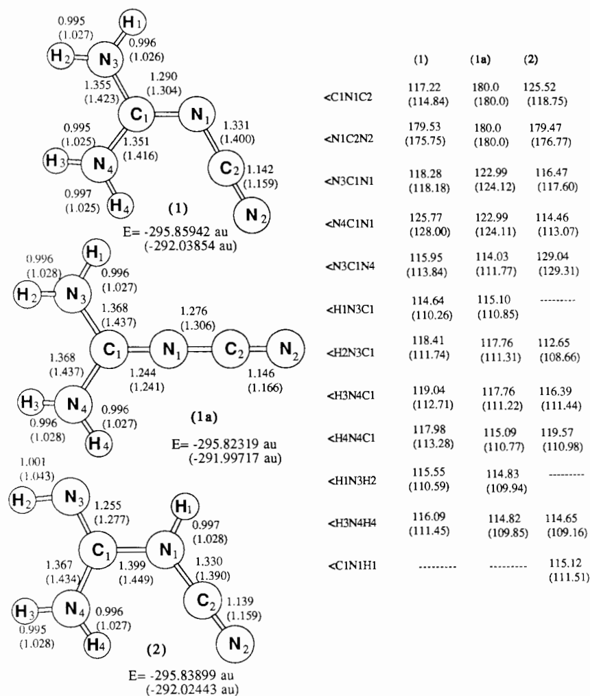
Figure 1. Structures of cyanoguanidine ( 1 ), linear cyanoguanidine transition state ( 1a ) and the isomer of cyanoguanidine ( 2 ) calculated at the HF/6-31G* level (values in parentheses are HF/STO-3G)
