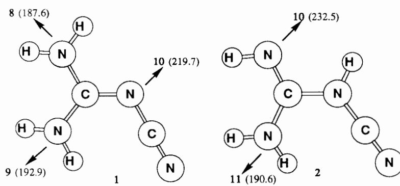
Figure 4. Proton affinities of amino and imino nitrogens in 1 and 2 (HF/6-31G*, kcal mol -1 )
