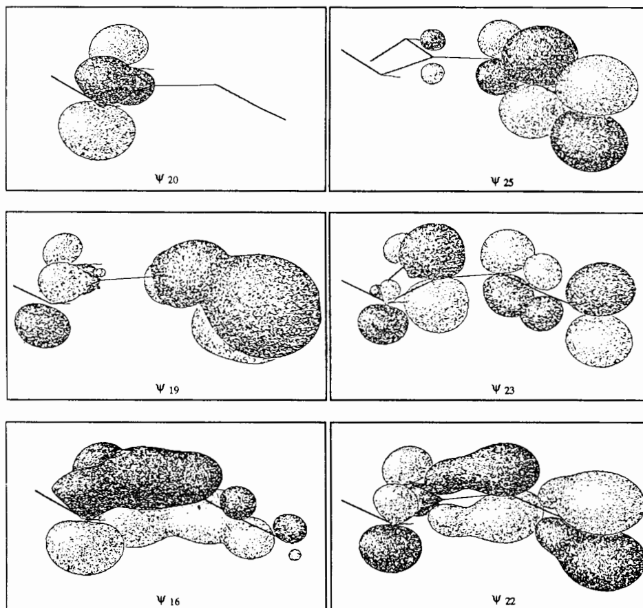
Figure 3. Molecular orbital plots of ground-state dicyandiamide (STO-3G)
